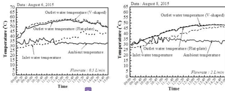
Figure 7 Inlet and outlet water temperature.
