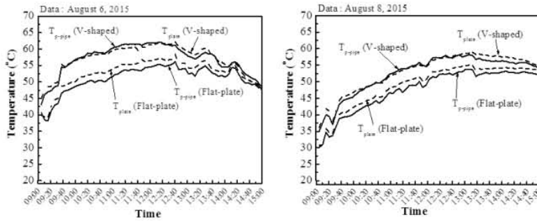
Figure 8 Surface temperature of the absorber plate.
