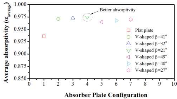
Figure 4 Average absorptivity of absorber plates.
