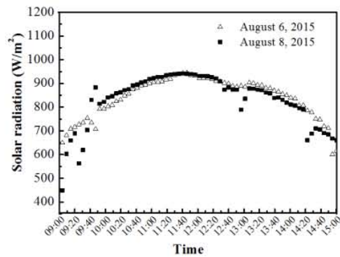
Figure 6 Solar radiation.
