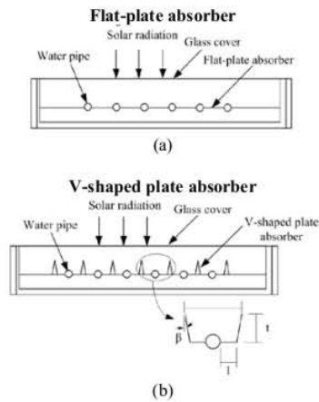
Figure 2 Cross sectional view of solar water heater.
